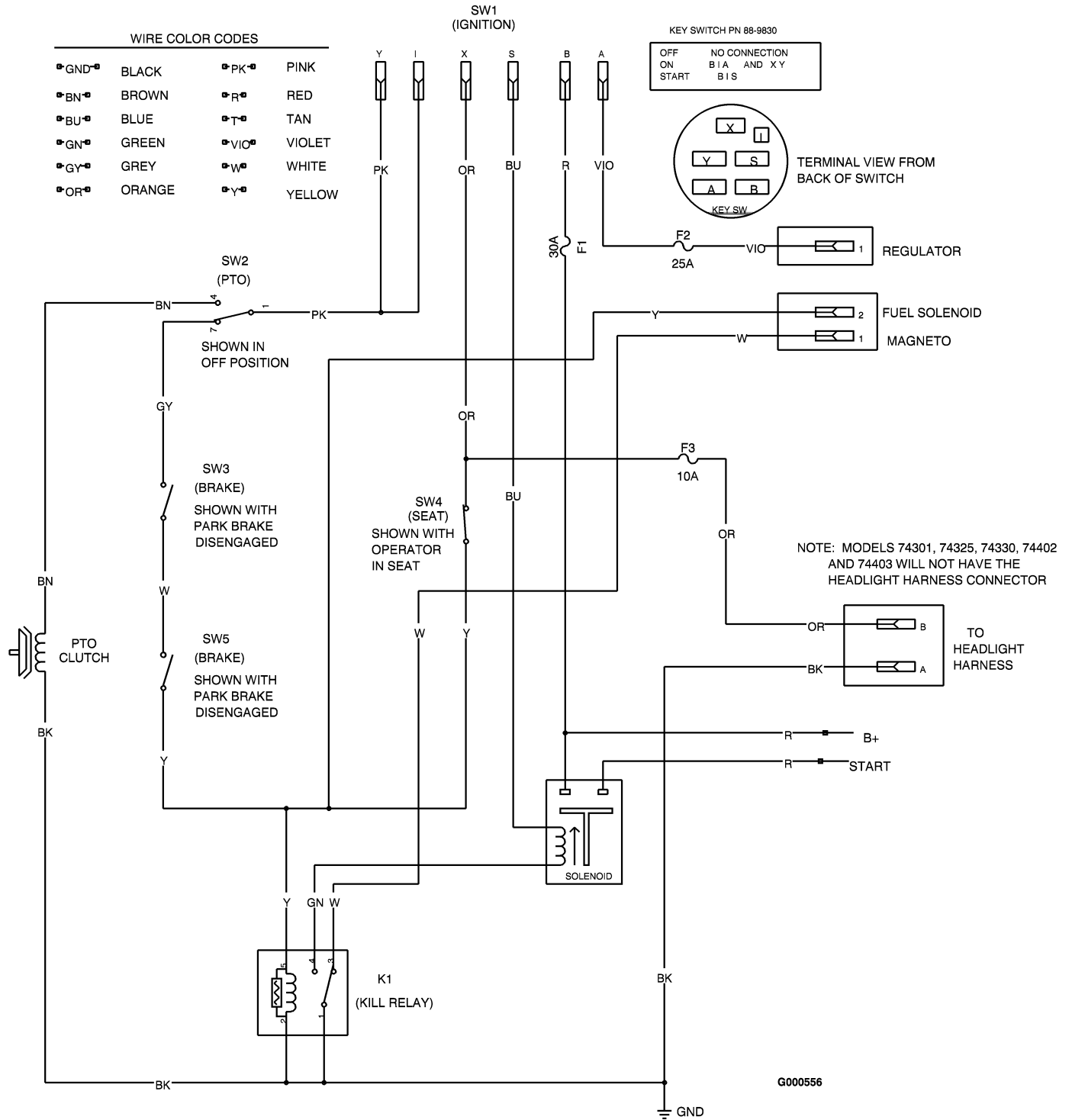
Electrical Diagram (Rev. A)
