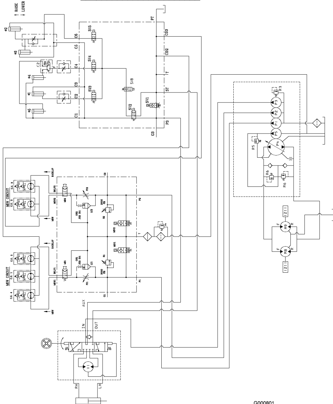
Hydraulic schema, Model 03806 (Rev. -)
