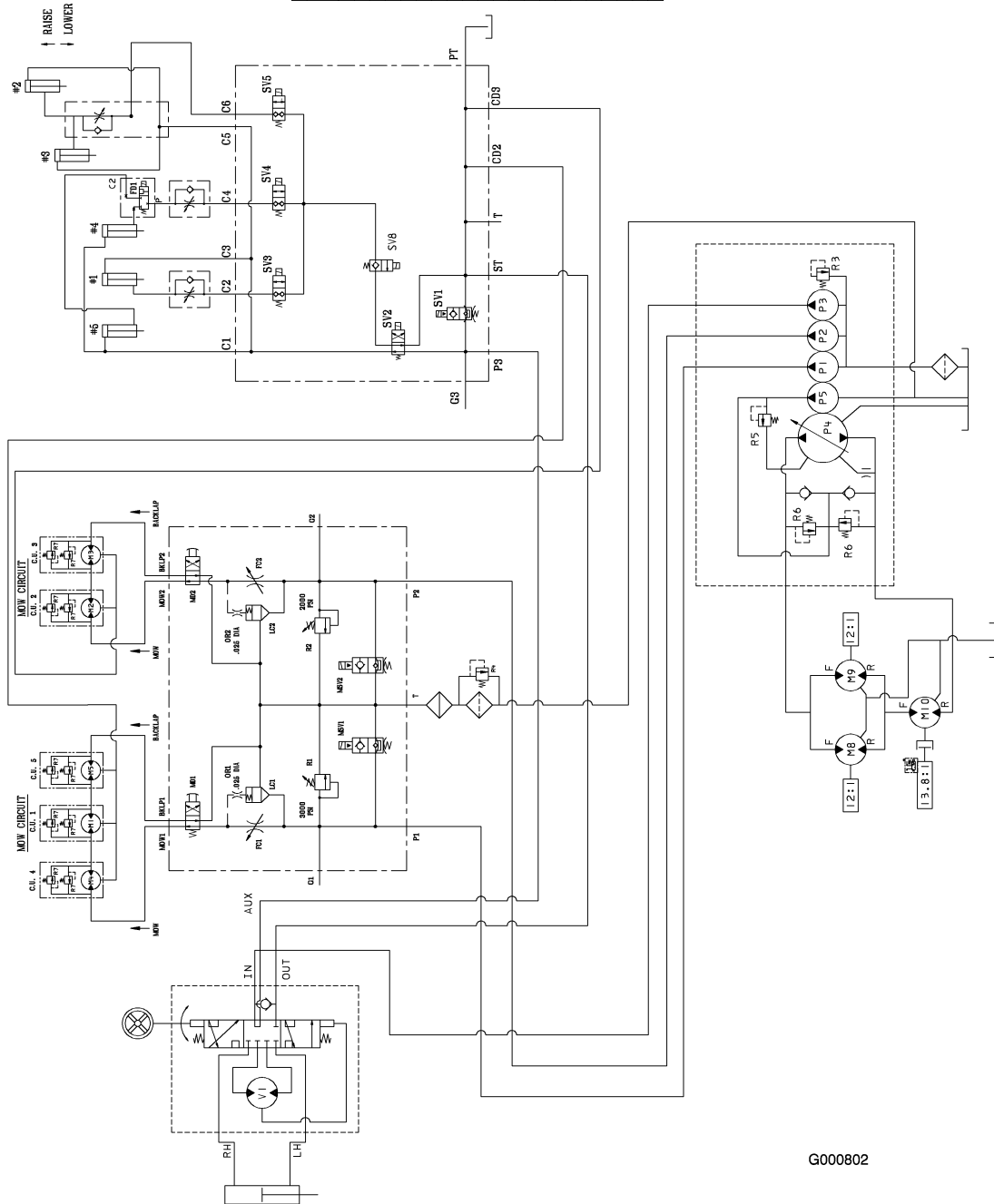
Hydraulic schema, Model 03807 (Rev. -)
