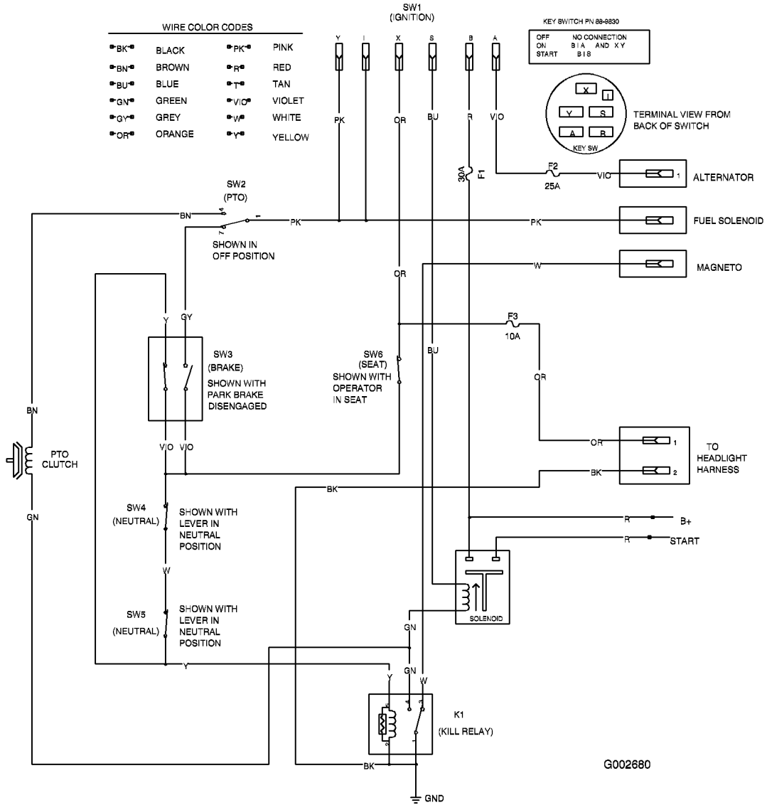
Electrical Schematic (Rev. B)
