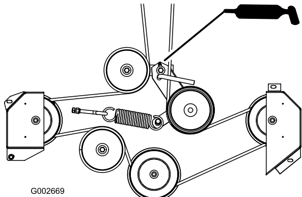
Figure 22 Top View
