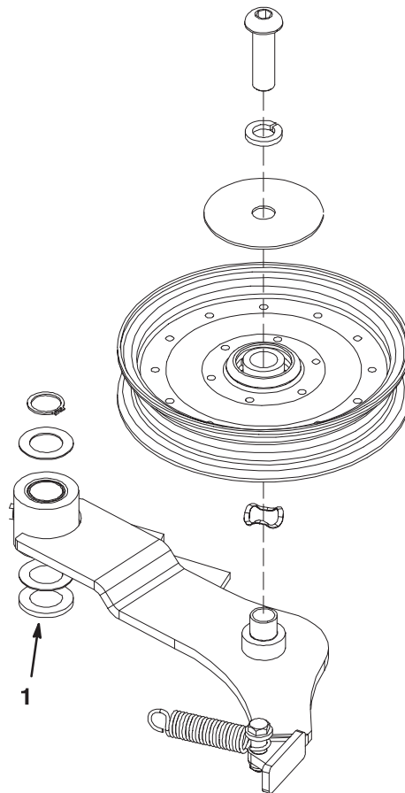
Pulley Mounted Above Idler Arm
