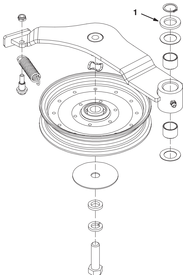
Pulley Mounted Under Idler Arm
