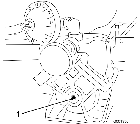
Figure 41 Pompe (ne lubrifiez pas excessivement)
