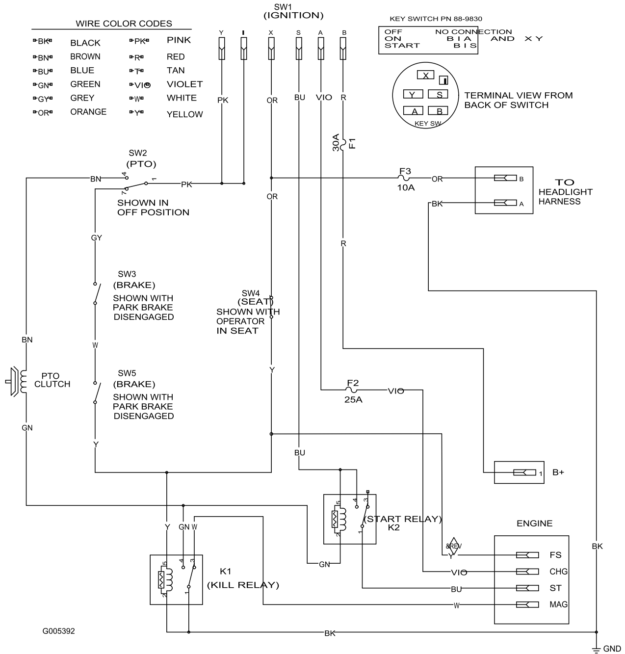
Electrical Diagram (Rev. A)
