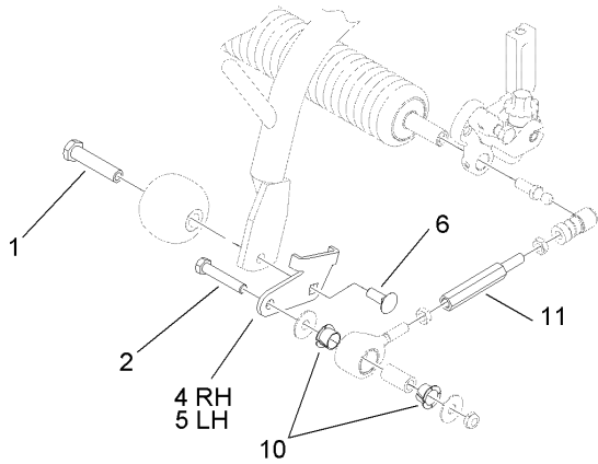
FRONT C/U GROOMER EXTENSION ASM POST 2007 CONFIGURATION (RIGHT ARM SHOWN)
