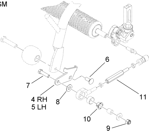
FRONT C/U GROOMER EXTENSION ASM PRE 2007 CONFIGURATION (RIGHT ARM SHOWN)
