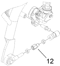
REAR C/U GROOMER EXTENSION ASSEMBLY ITEMS 4,5,6,7,8,9,11 NOT USED
