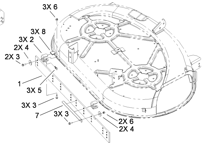
42 INCH DECK
