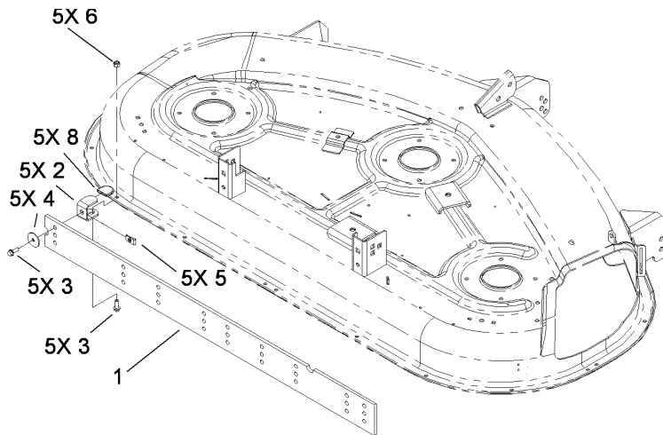
50 INCH DECK
