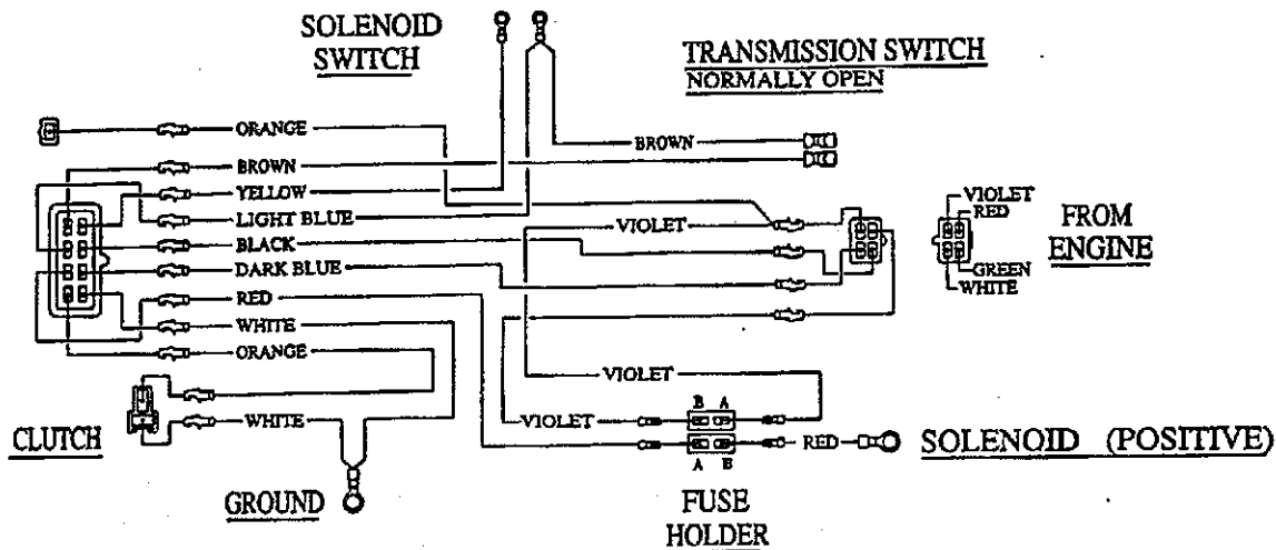
Engine Deck Wiring Diagram
