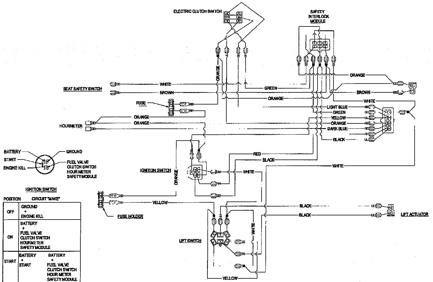
Console Wiring Diagram
