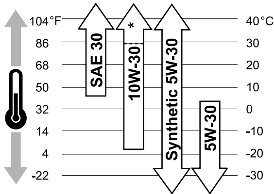
Figure 26 Viscosity Grades
