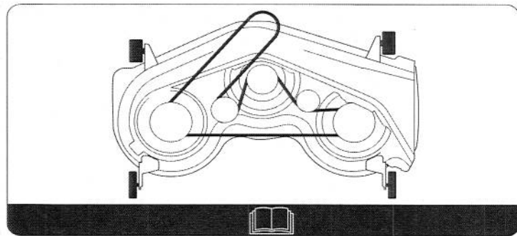
Part No. 112-1273
