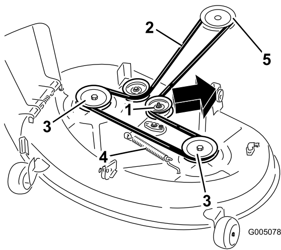
Figure 58 Mower Decks with 2 Blades
