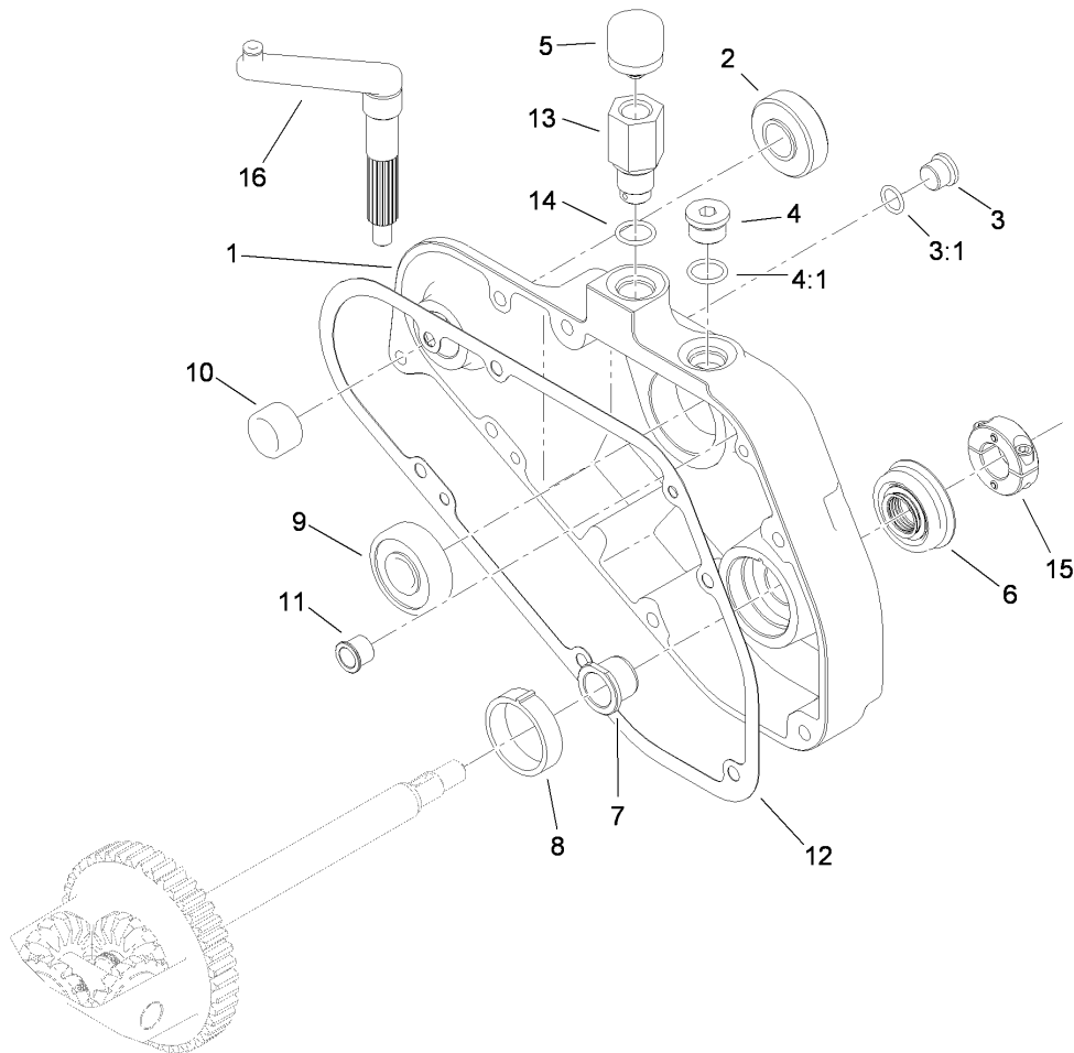
Gearbox Cover Assembly No. 117-1461
