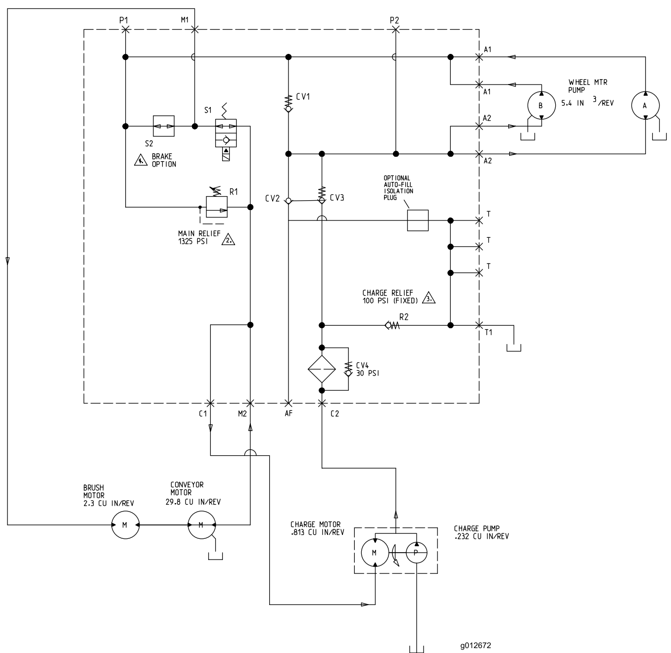
Hydraulic Schematic (Rev. 1)
