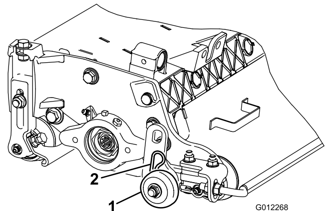
1. Transport roller assembly 2. Cotter pin
