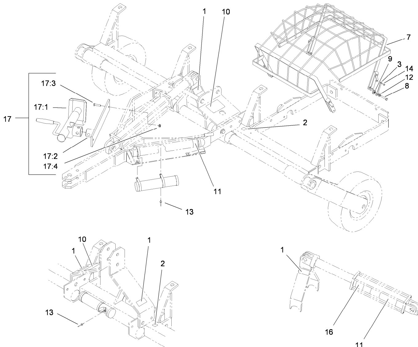
686 AERATOR HITCH
