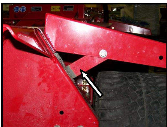
Figure 15: Fender Bracket Installed
