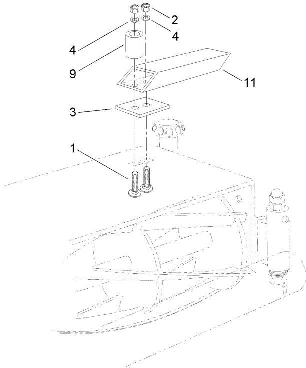
TM549 Cutterhead 1 Shown Cutterhead 6 opposite hand.
