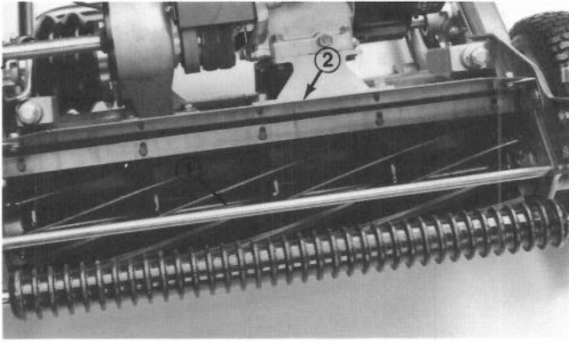
Figure 16 1. Crossbar 2. Shield
