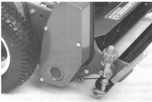
Figure 13 1. Height-of-cut brackets
