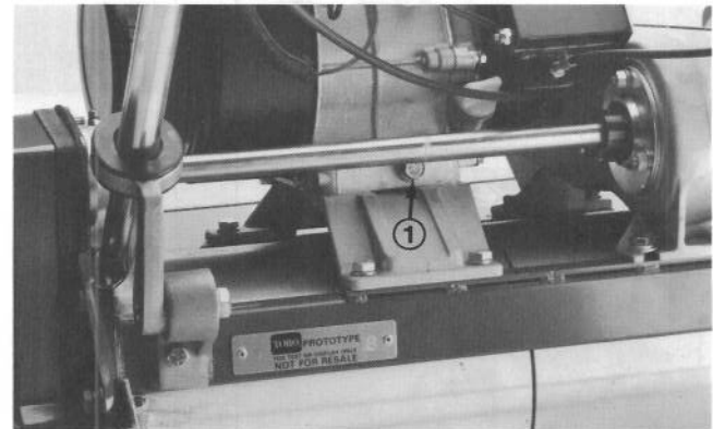
Figure 25 1. Drain plug
