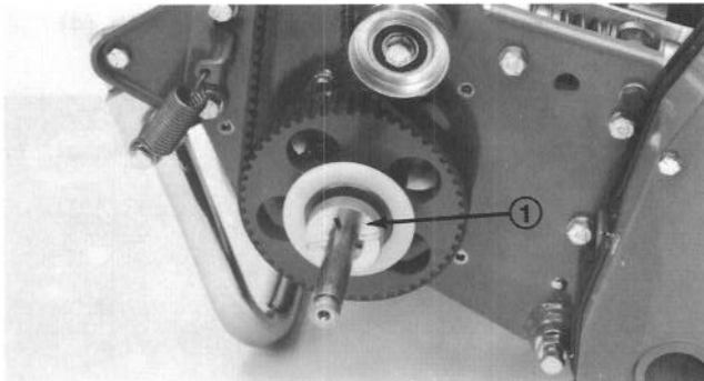
Figure 6 1. Locking collar
