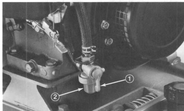
Figure 35 1. Shut off valve 2. Bowl
