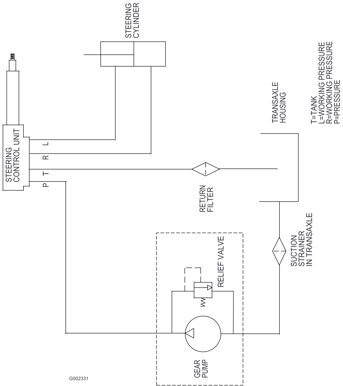
Hydraulik (Rev. A)
