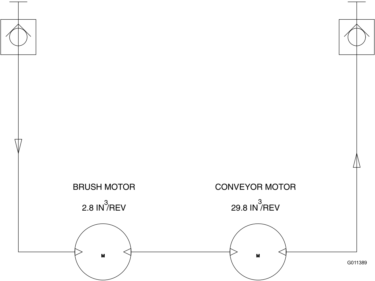
Hydraulic Schematic (Rev. A)
