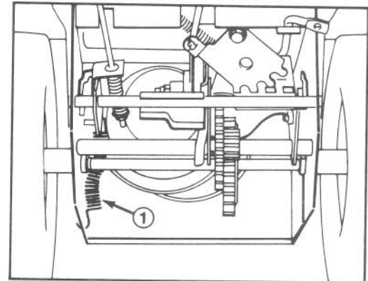
Figure 25 1. Ressort
