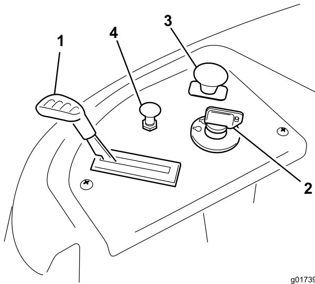
Figure 6 Control Panel
