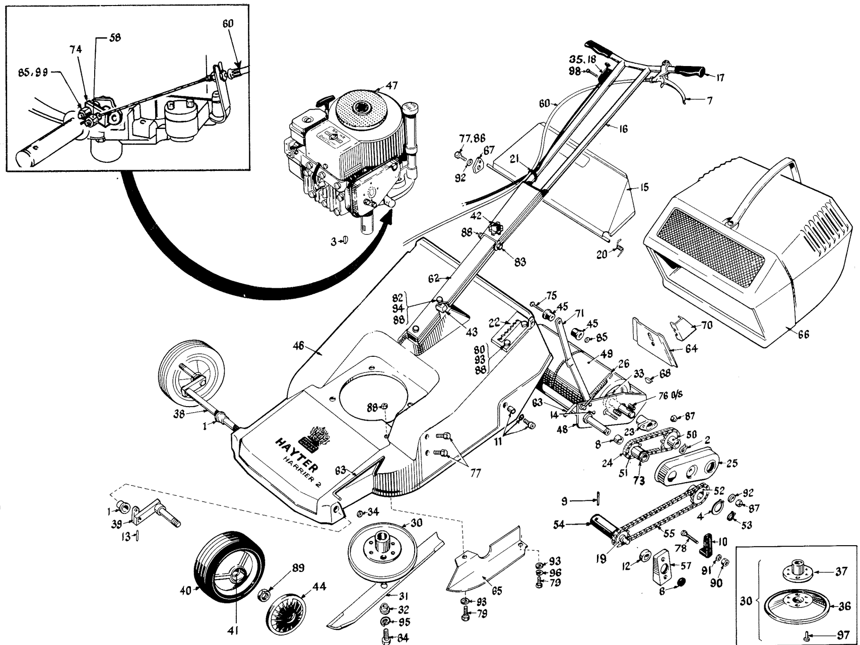
Fig. 3 Mainframe Assembly
