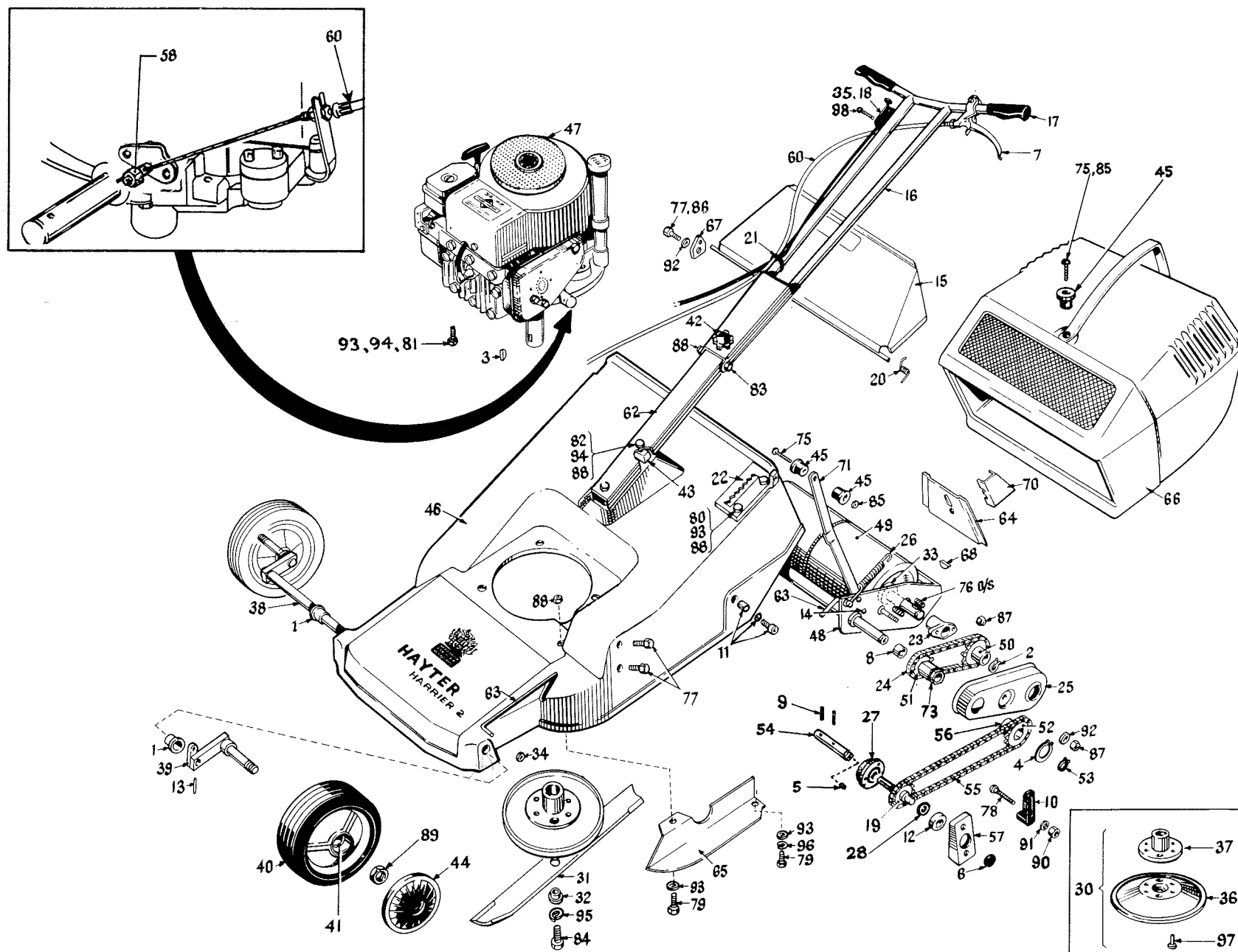
Fig. 3 Mainframe Assembly
