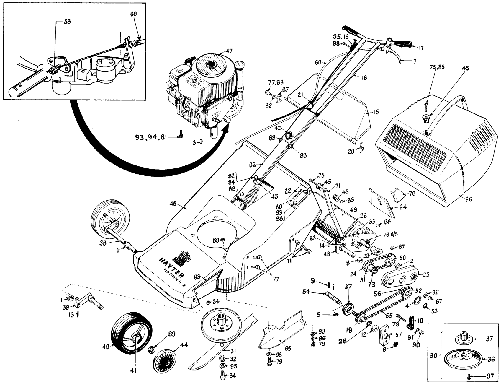
Fig. 3 Mainframe Assembly
