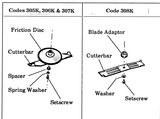
Fig 2. CUTTERBAR ASSEMBLY
