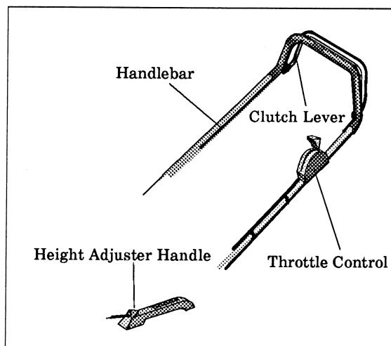
Fig 1 OPERATOR CONTROLS
