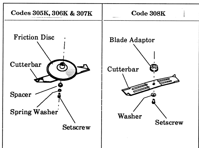
Fig 2. CUTTERBAR ASSEMBLY
