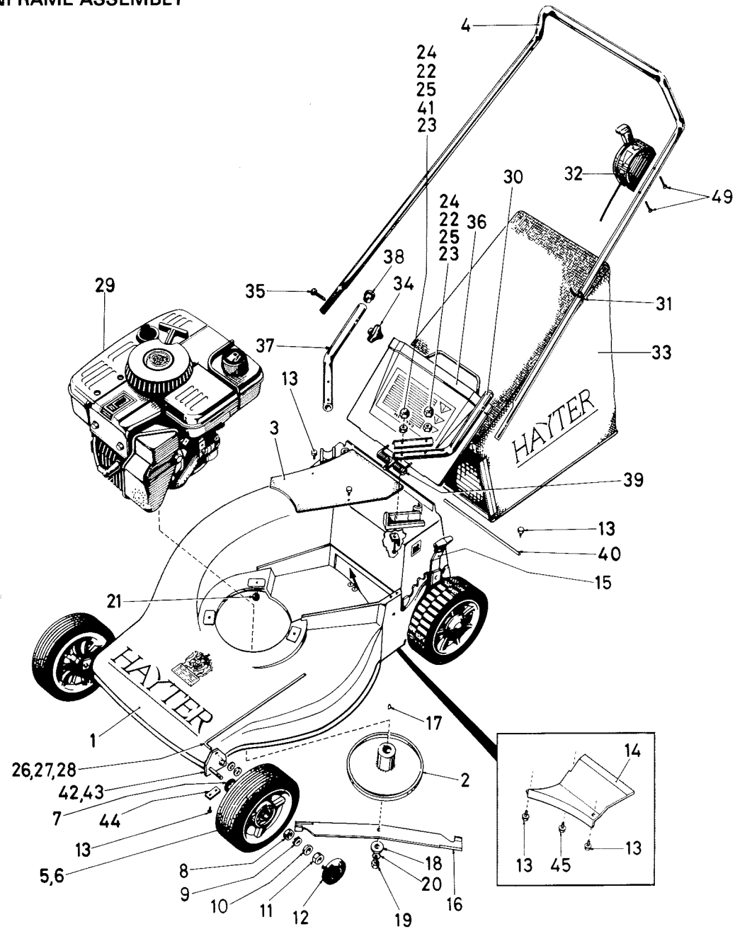
Fig. 1 330 MAINFRAME ASSEMBLY
