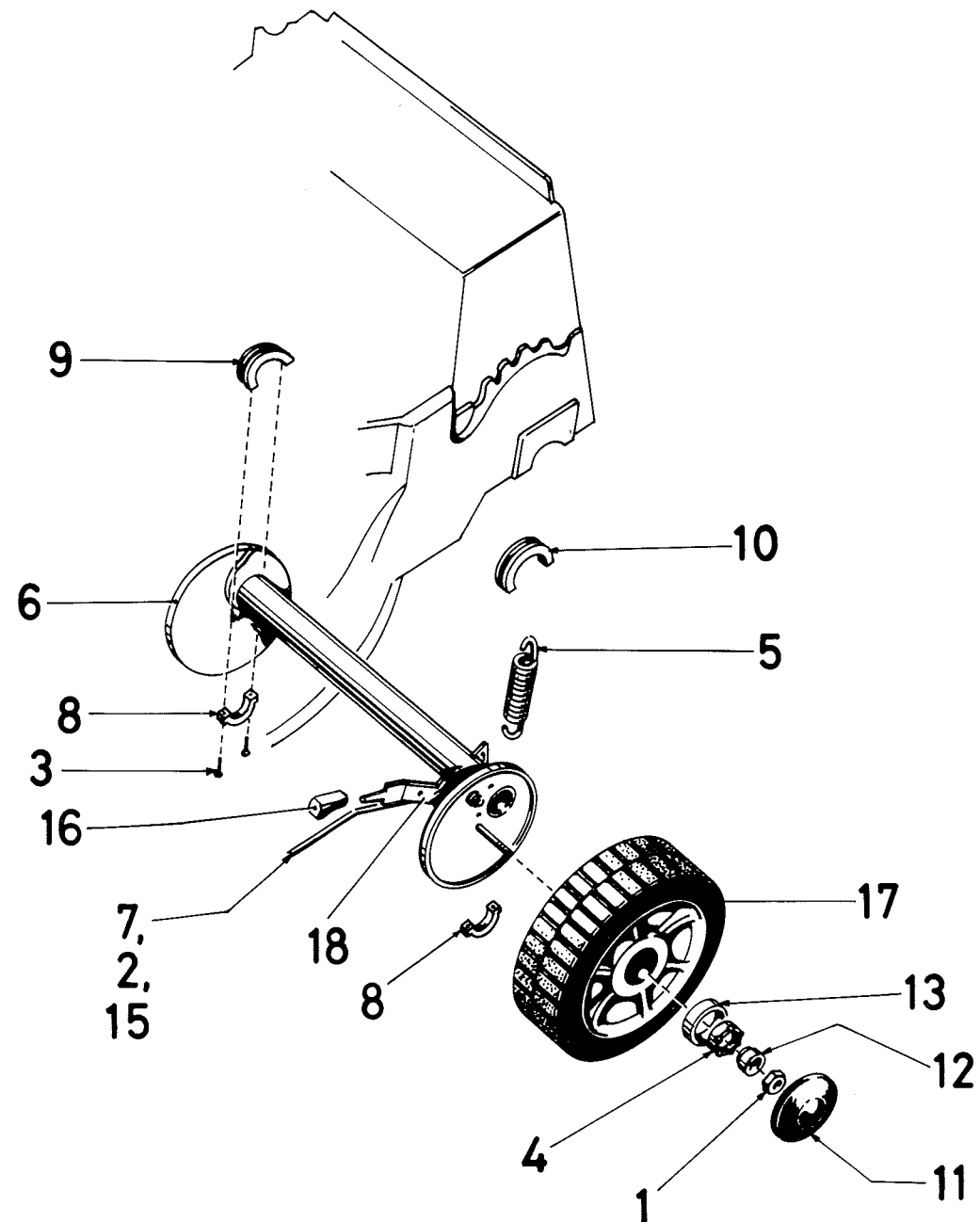
Fig. 2. 330 REAR AXLE ASSEMBLY
