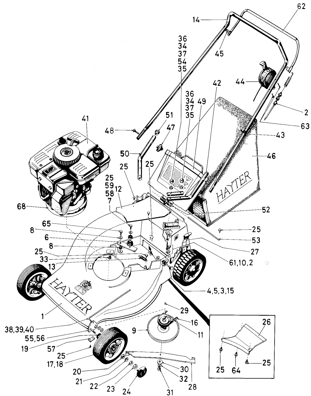
Fig. 3. 331 MAINFRAME ASSEMBLY
