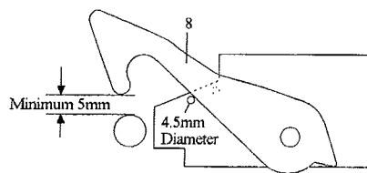
(A) Front RH Latch Modification Raised Position (LH Opposite)
