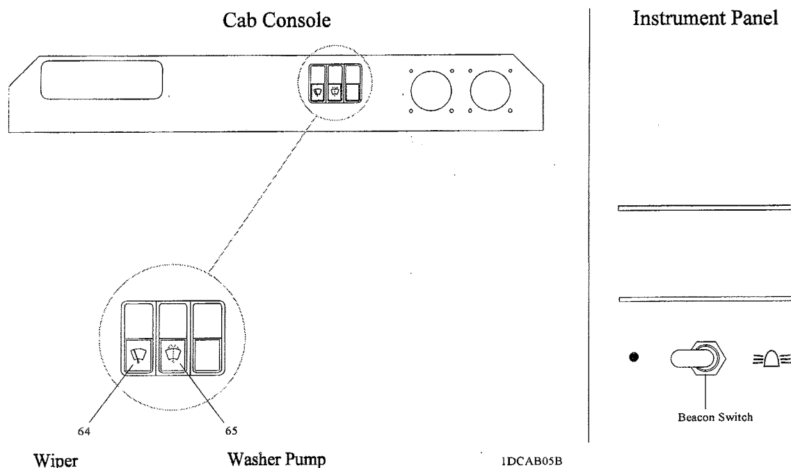
Fig. 14. Switch controls.
