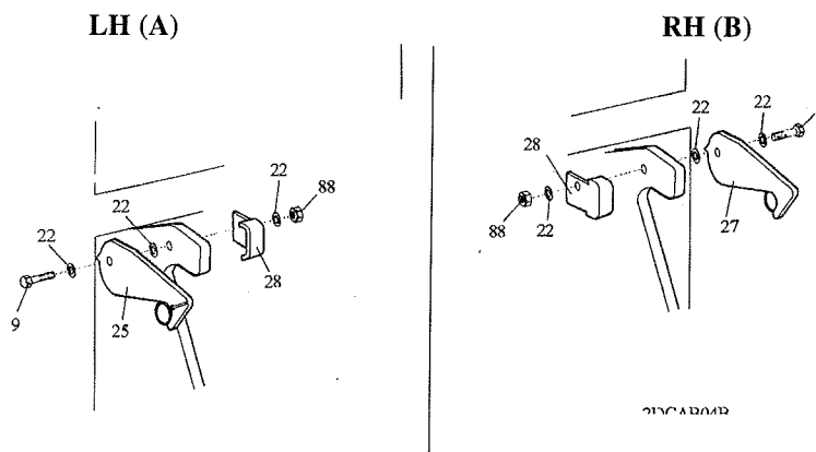
Fig. 4. Wing arm transport latches.
