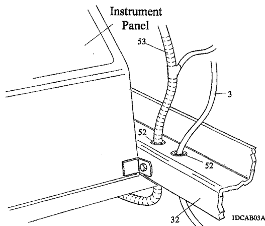
Fig. 7. Wire routing
