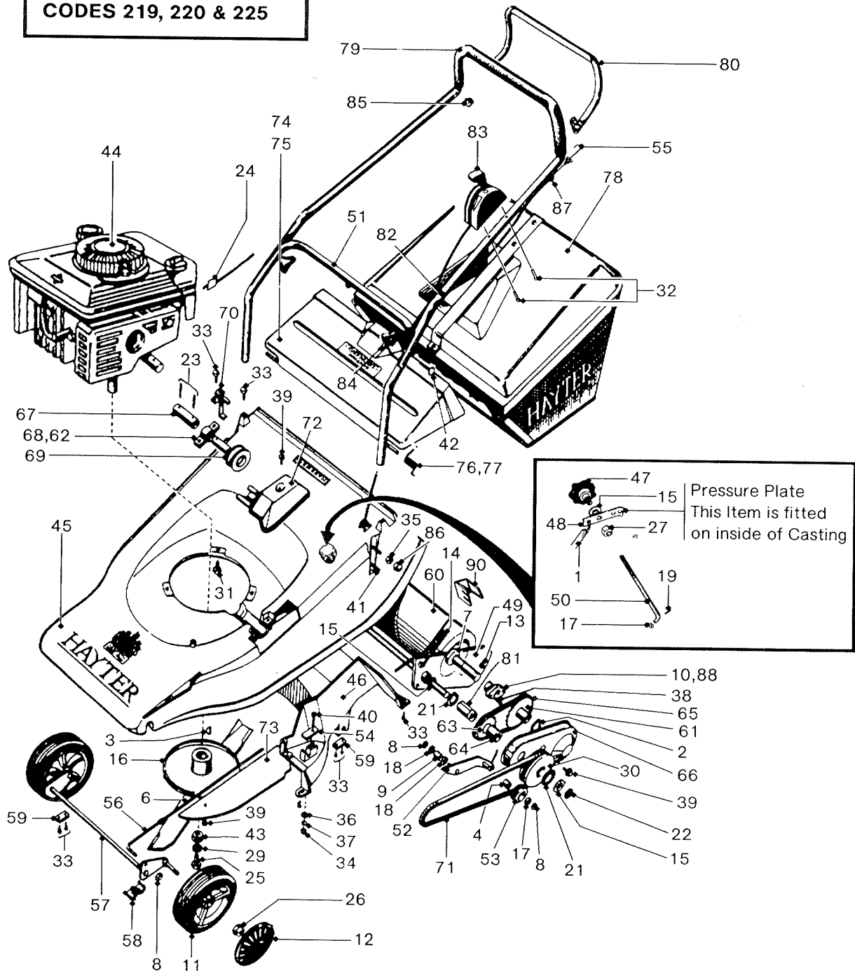
FIG. 1 SELF PROPELLED MOWER ASSEMBLY
