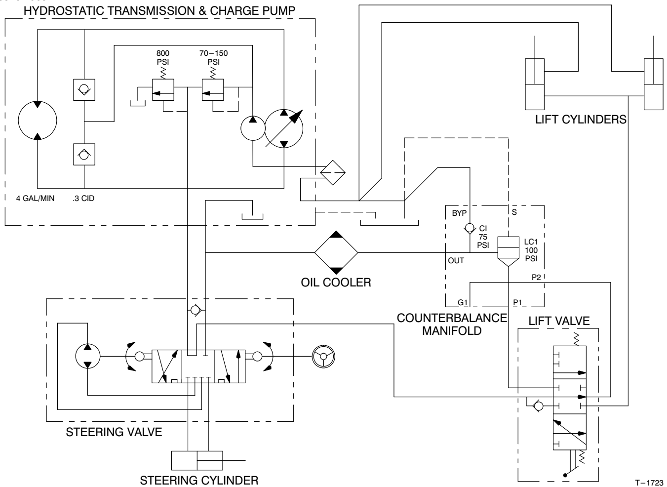
HYDRAULIC SCHEMATIC
