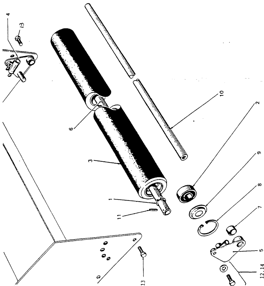
REAR ROLLER ASSEMBLY
