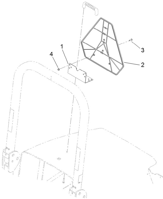
GROUNDMASTER 3280 INSTALLATION
