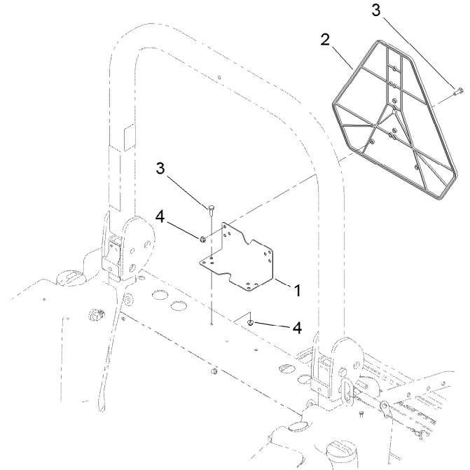
GROUNDMASTER 7200/7210 INSTALLATION
