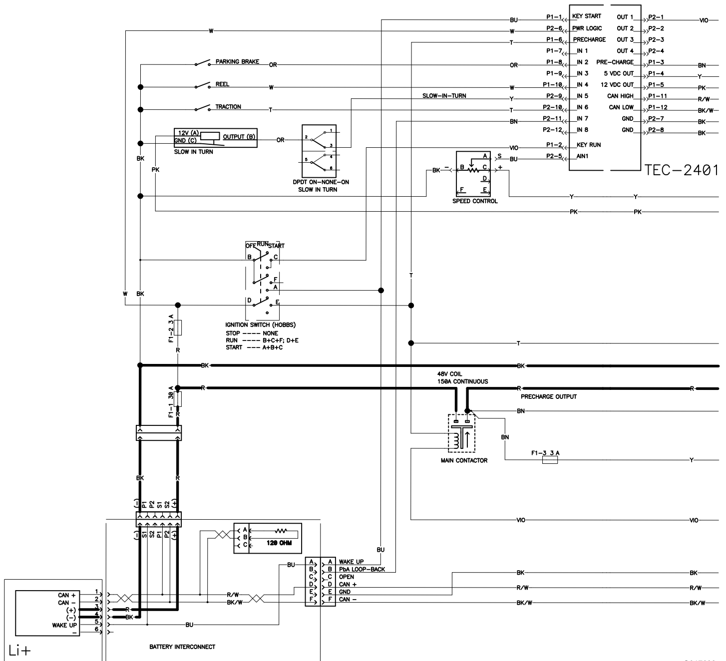
Electrical Schematic, Part 1 (Rev. A)
