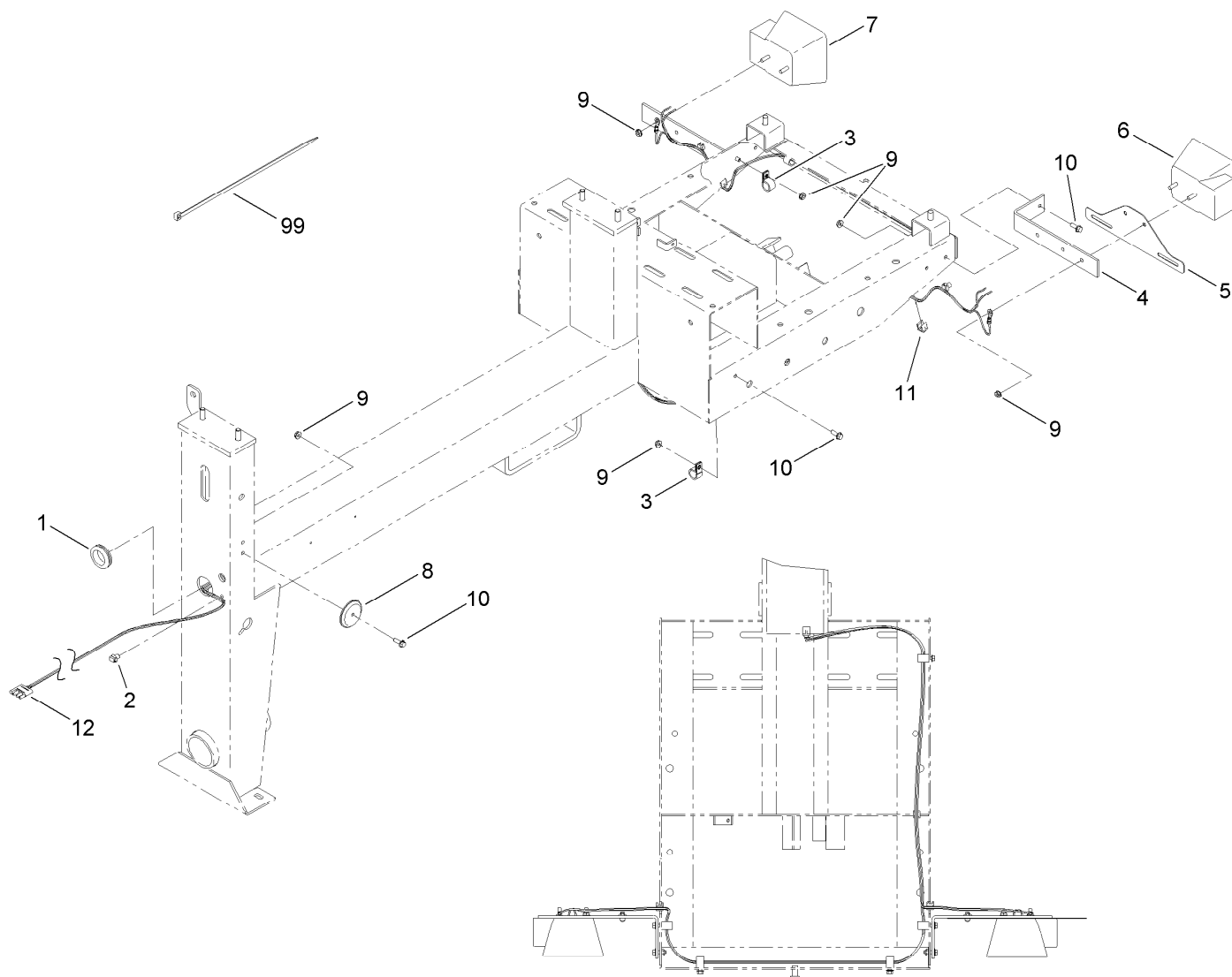
VIEW OF HARNESS ROUTING UNDER FRAME
