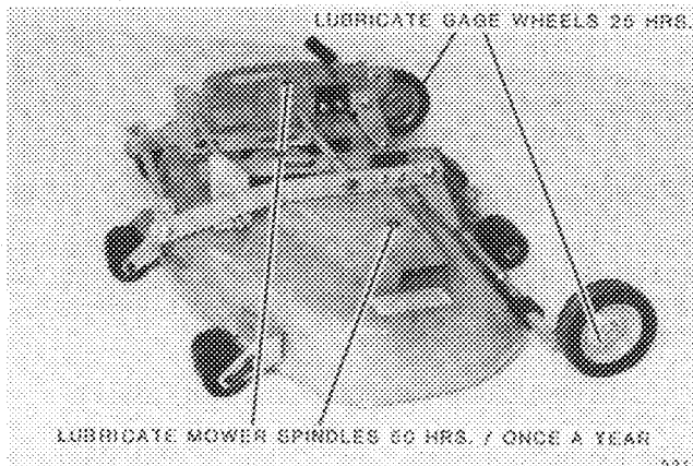
FIG. 16. Three Blade Mower Lubrication Fittings
