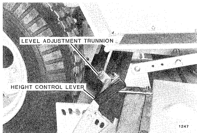
FIG. 10. Level Adjustment
