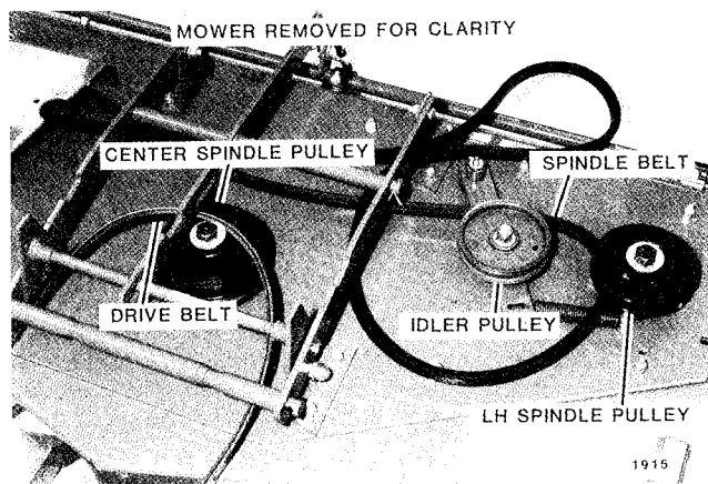
FIG. 17 Drive Belt Removal
