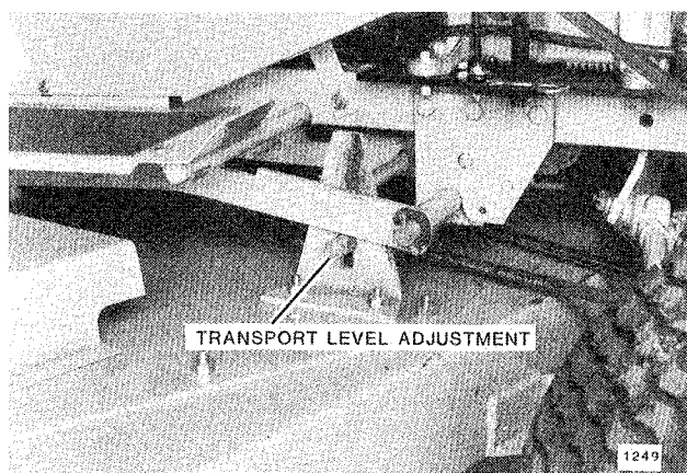
FIG. 13. Transport Level Adjustment
