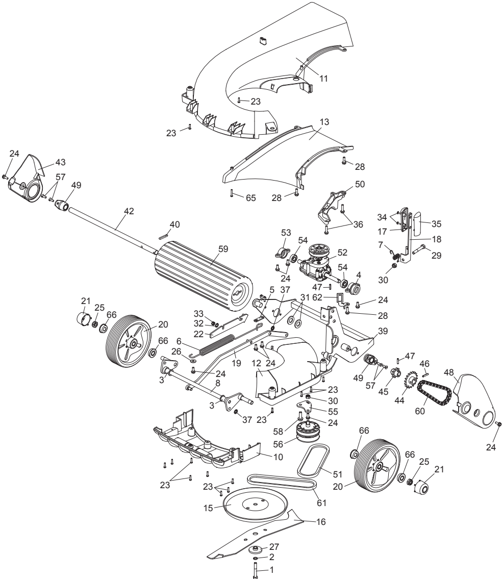
Lower Mainframe
