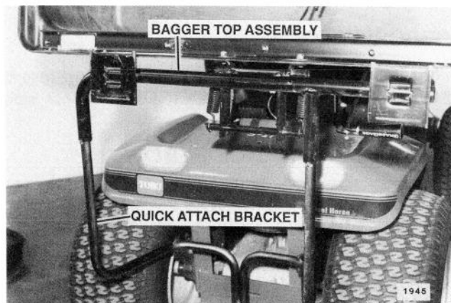
FIG. 9. Install Bagger Top on Quick Attach Bracket
