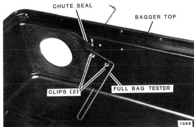
FIG. 6. Install Full Bag Tester Through Bagger Top
