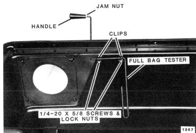
FIG. 7. Secure Full Bag Tester And Install Handle
