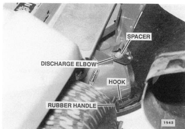
FIG. 3. Rear Discharge Chute Mounting
