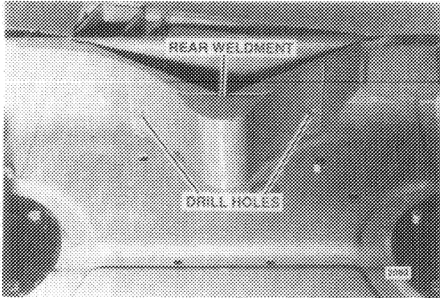
FIG. 1 Install Rear Weldment
