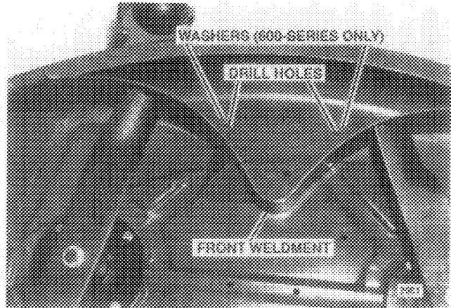
FIG. 2 Install Front Weldment
