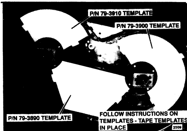
FIG. 5 Kicker Template Location on Deck
