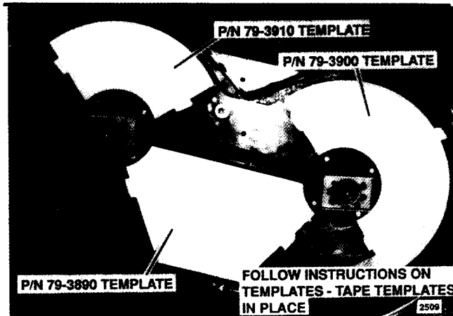
FIG. 5 Kicker Templates Located on Mower Deck
