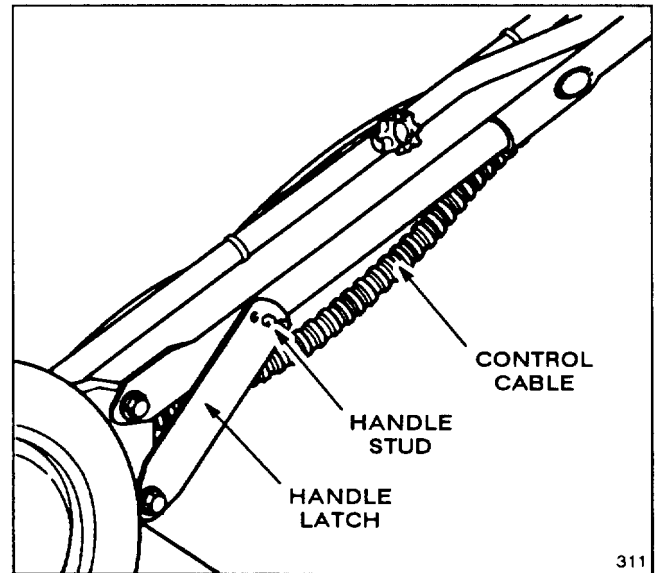
Self-propelled model
