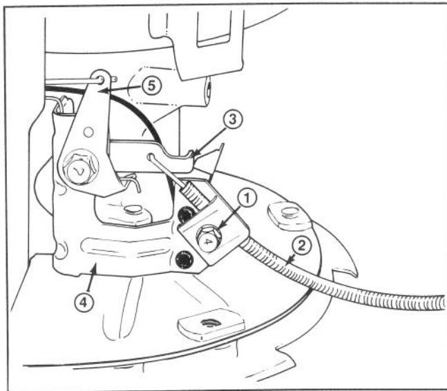
OFF (engine kill) position
