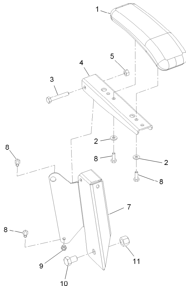
LH Armrest Assembly
