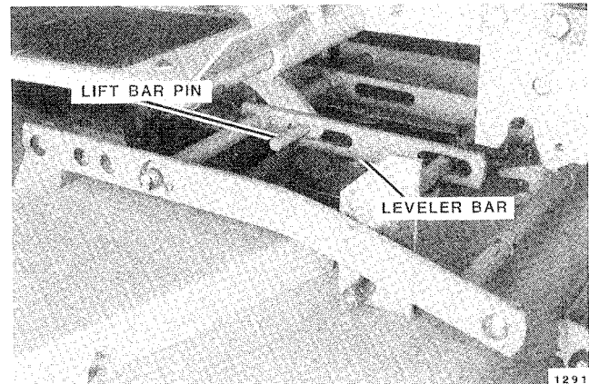
FIG. 2. Align Pin with Slot
