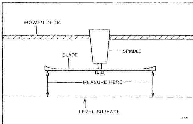
FIG. 13. Mower Level Measurement
