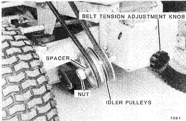
FIG. 11 Mower Front Idler Pulleys
