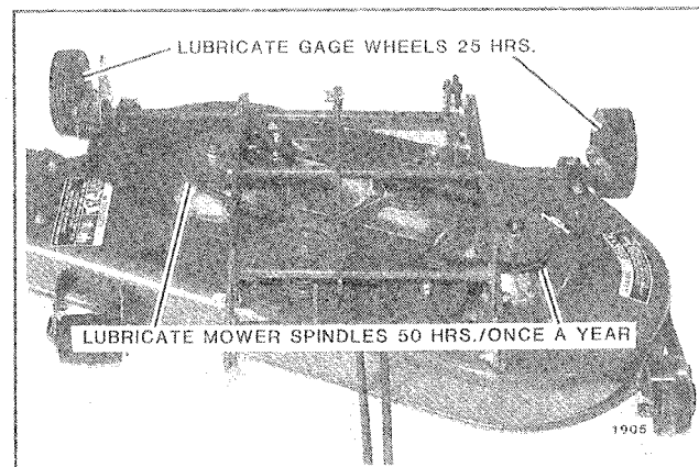
FIG. 17. Mower Lubrication Fittings
