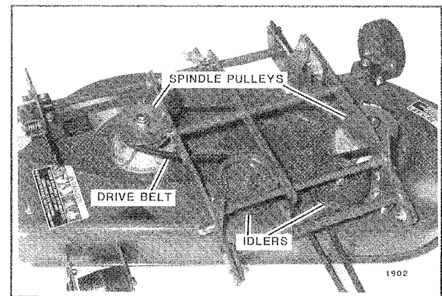
FIG. 9 Mower Drive Belt
