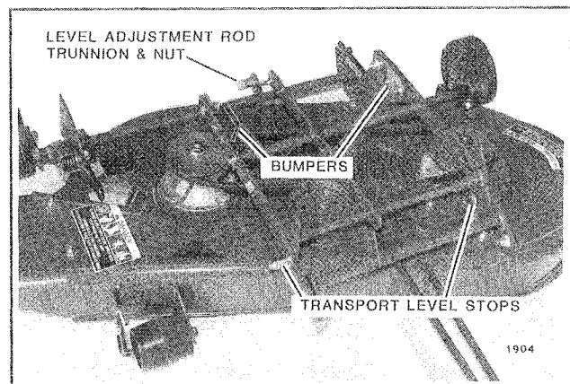
FIG. 15. Mower Adjustments
