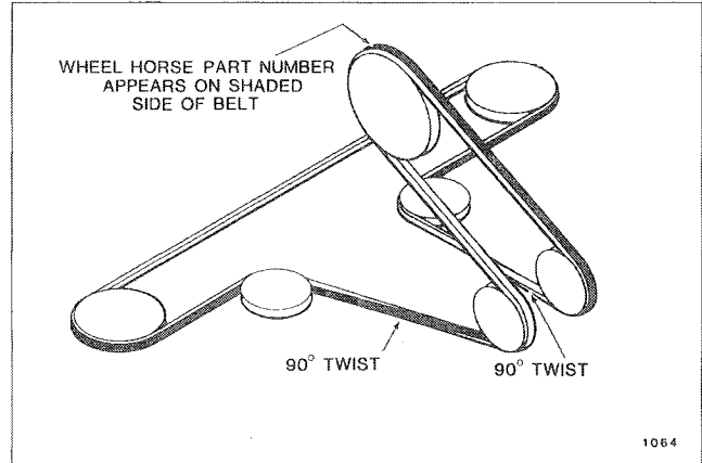
FIG. 8 Mower Drive Belt Routing
