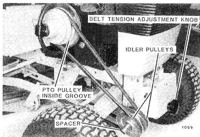
FIG. 10 Mower Front Pulleys
