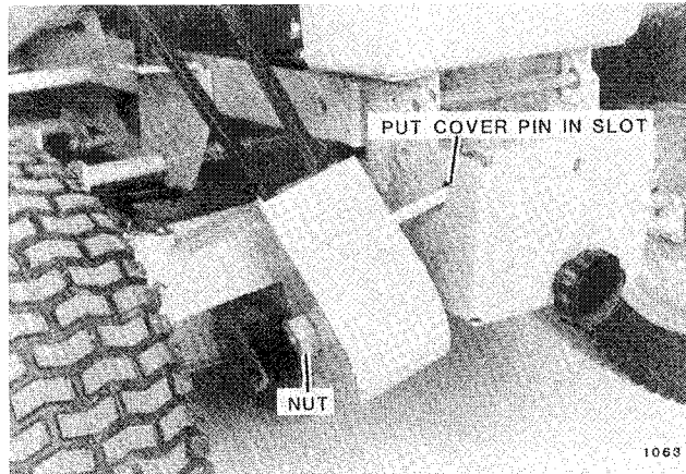
FIG. 12. Install Pulley Support Cover
