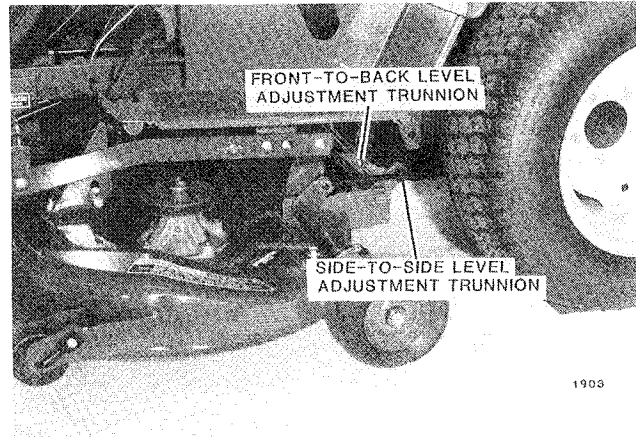
FIG. 14. Level Adjustments
