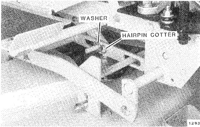
FIG. 5. Secure Mower to Tractor Lift Bar Pin
