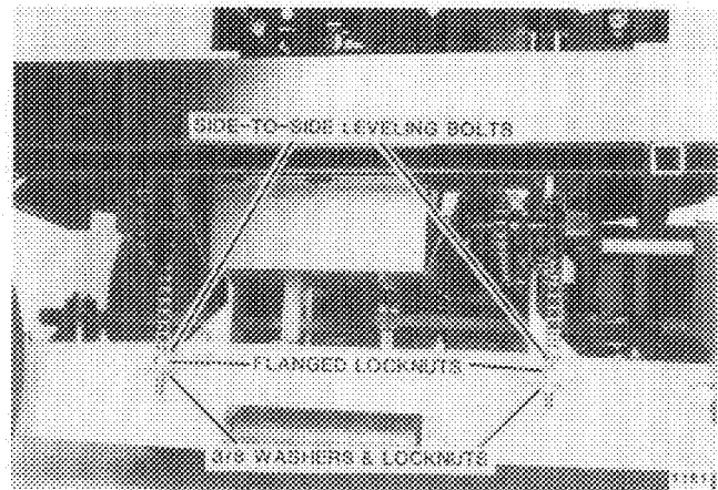
FIG. 6. Install Side-To-Side Leveling Chain Bolts
