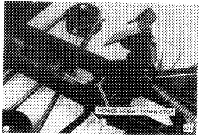
FIG. 14. Mower Height Down Stop
