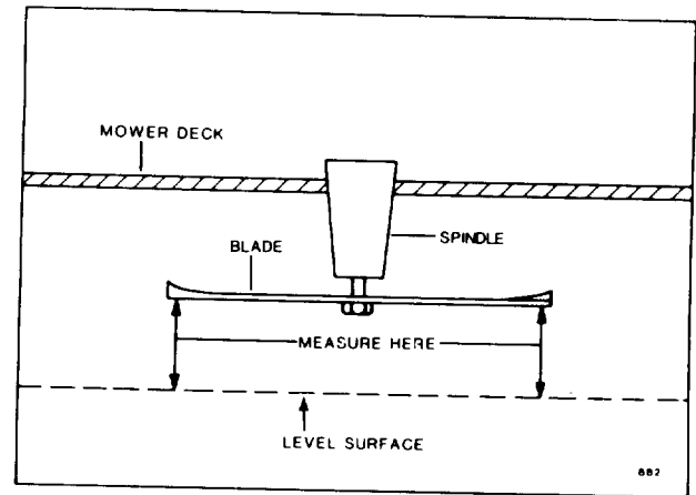
FIG. 10. Mower Level Measurement
